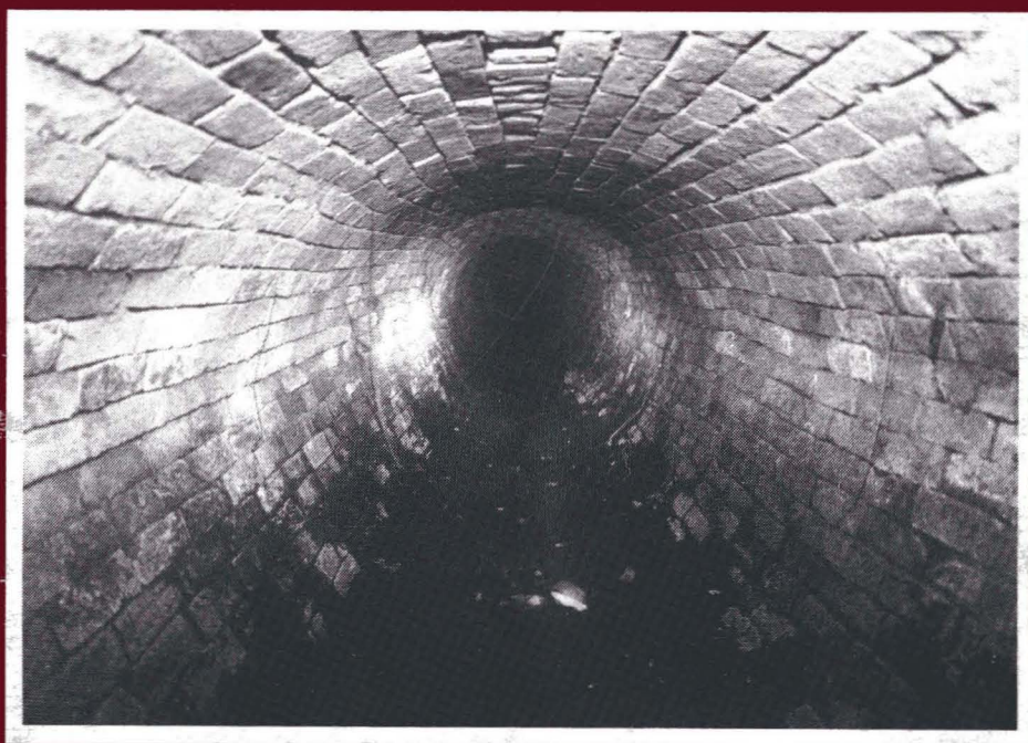
Brick barrel-drain of the 1820s, Parramatta.
